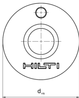
Sealing washer
