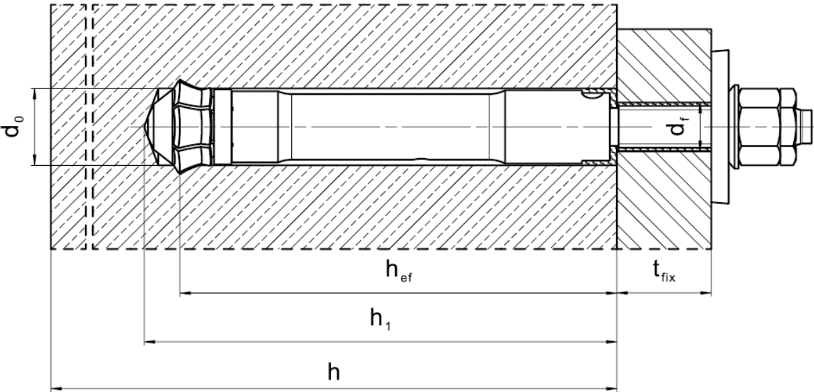
Figure A3: Pre-setting anchor HDA-P and HDA-PR (Prepositioning) with Filling Set
